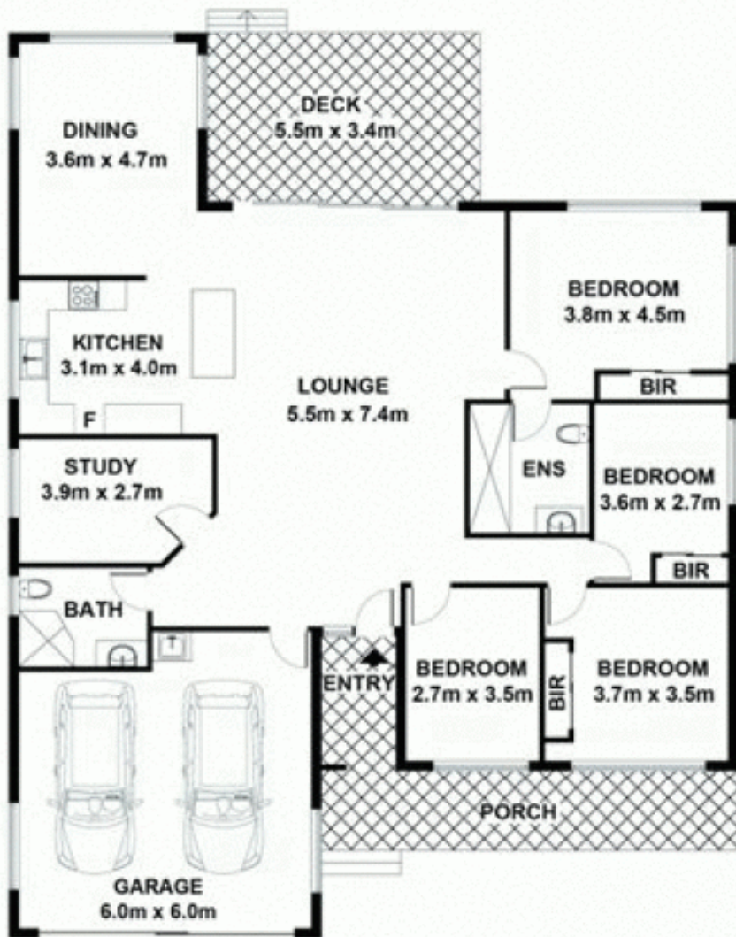
FLOOR PLAN
